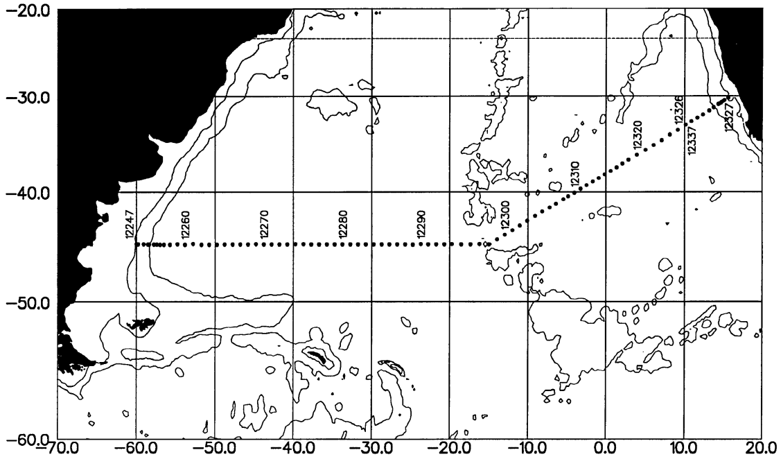
Figure 1: The A11 cruise track defined by CTD/Rosette stations. Isobaths of 200m and 3000m are superimposed
