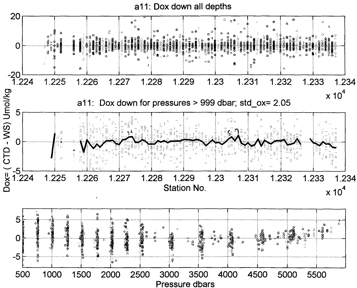
Figures 4a, 4b and 4c: CTD DQE
