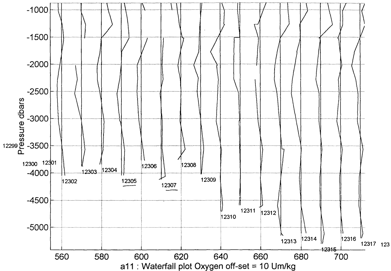
a11: Waterfall plot Dox=(CTD_dwn-WS); 10 Um/kg between stations
