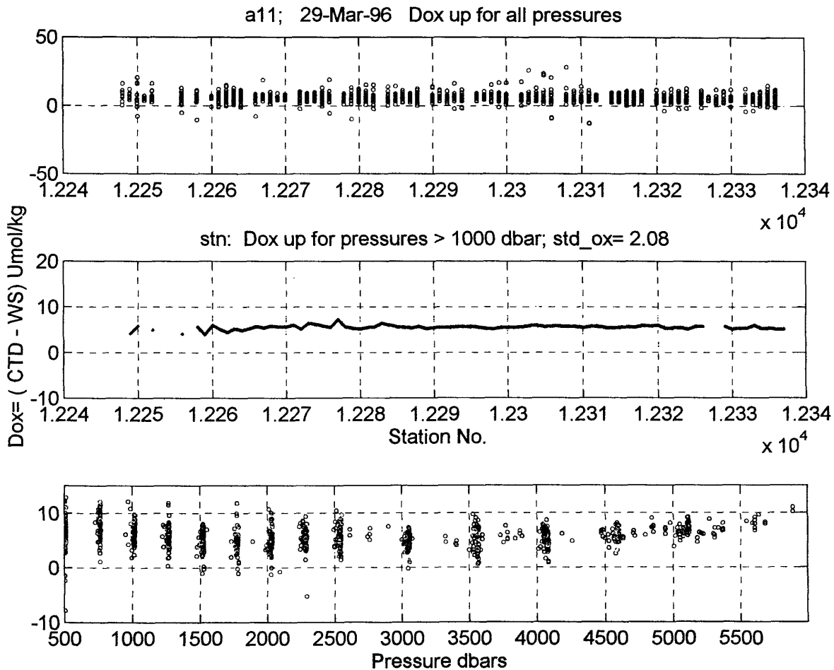
Figures 5a, 5b and 5c: CTD DQE
