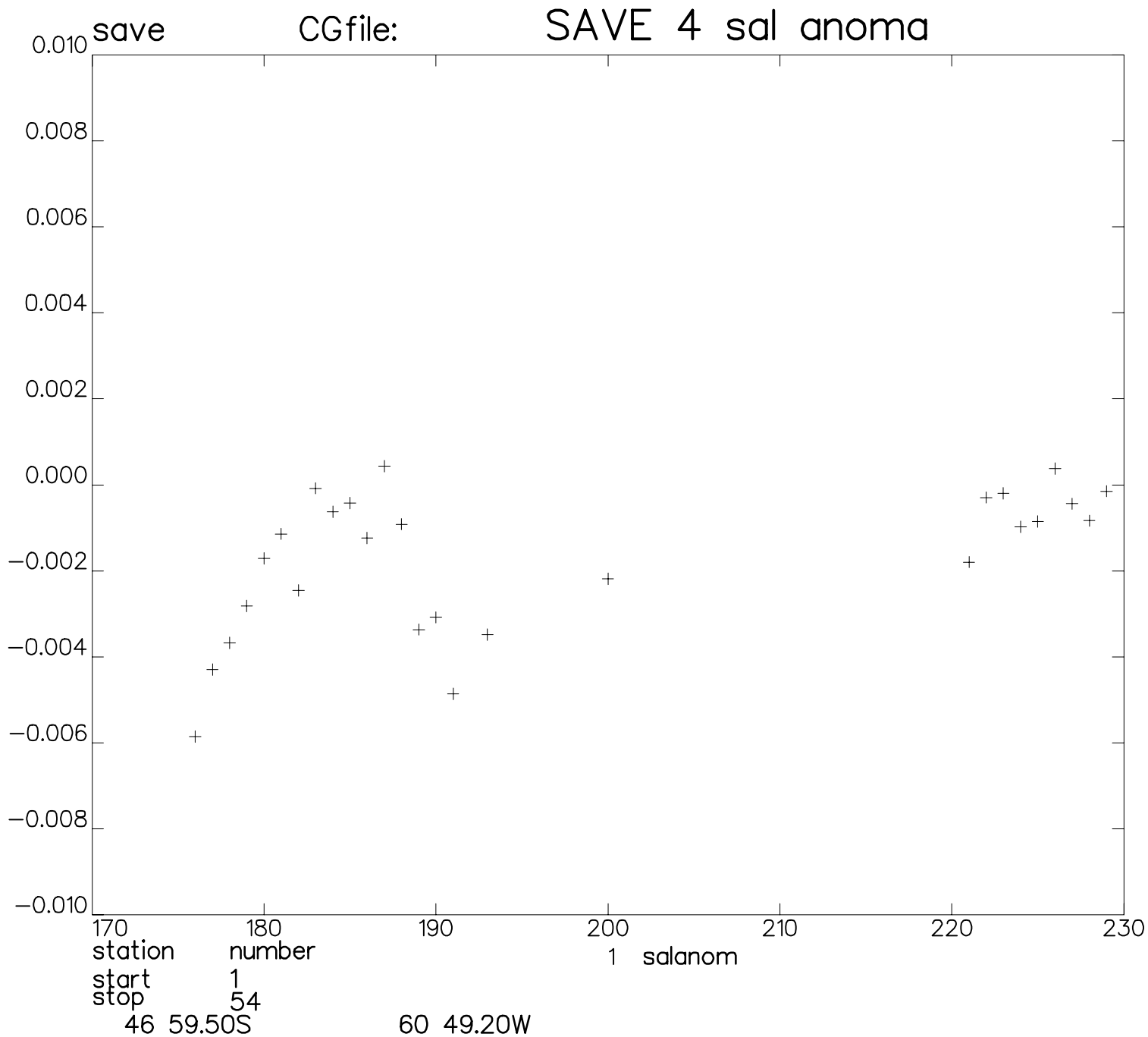
Figure 11: SAVE leg 4: station averages of anomaly of salinity relative to standard fits. Horizontal axis: station number. Vertical axis: salinity anomaly.
