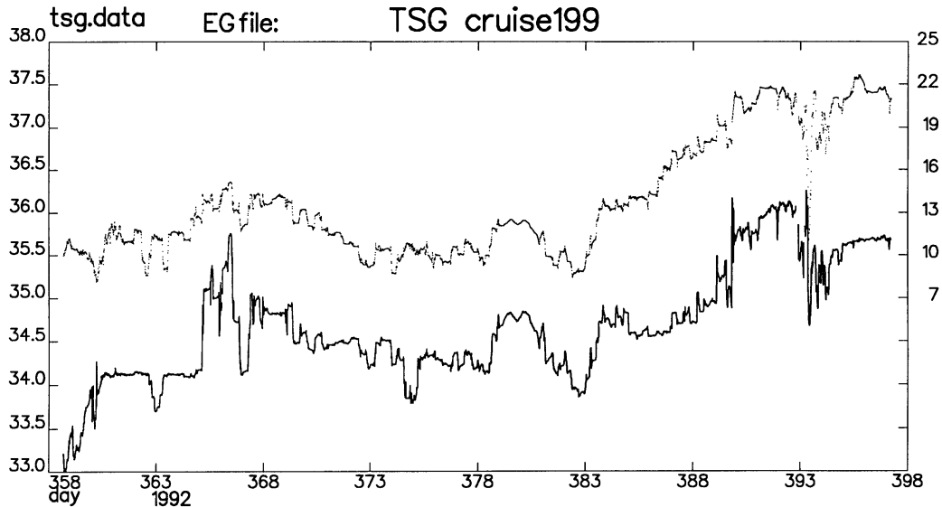
Figure 7: Surface salinity (bold) and temperature (broken) on cruise A11. The cruise begins on the Argentine shelf, passes through the Falkland current (day 363), the Brazil current retroflection (day 365), traverses the Subantarctic Zone until somewhere between day 386 and 390 it enters the subtropical gyre. The cruise ends in S.Africa
