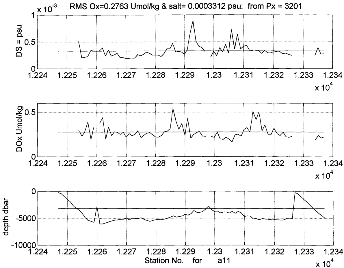
Figures 8a, 8b and 8c: CTD DQE
