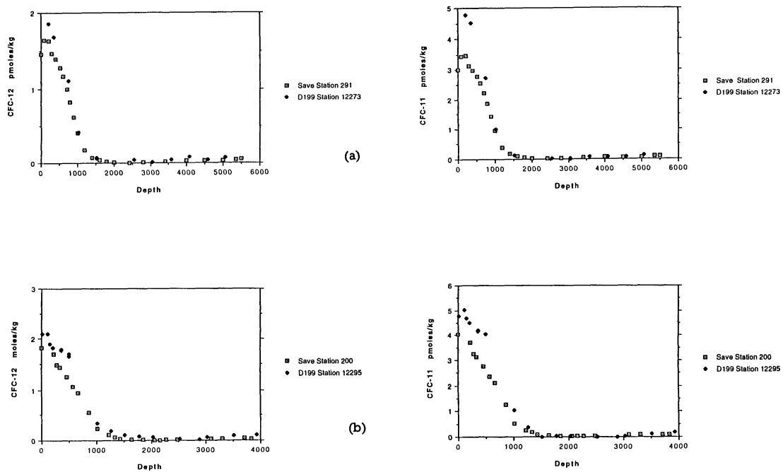
Figure 6: A comparison of CFC-11 and CFC-12 data from (a) SAVE station 291 and A11 station 12273 and (b) SAVE station 200 and A11 station 12295.
