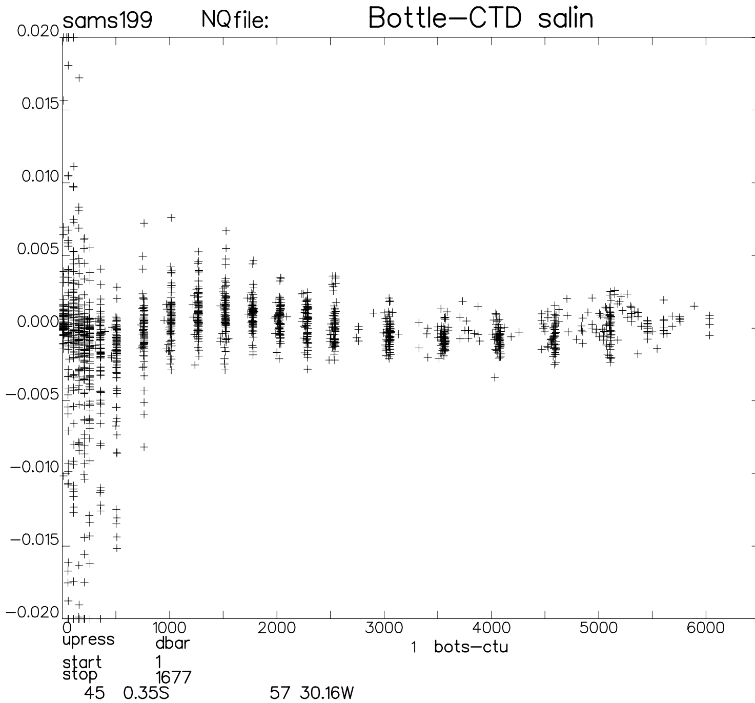
× Figure 10: This cruise: sample minus CTD salinity residuals for all samples flagged as good. Horizontal axis: pressure. Vertical axis: salinity residual.
