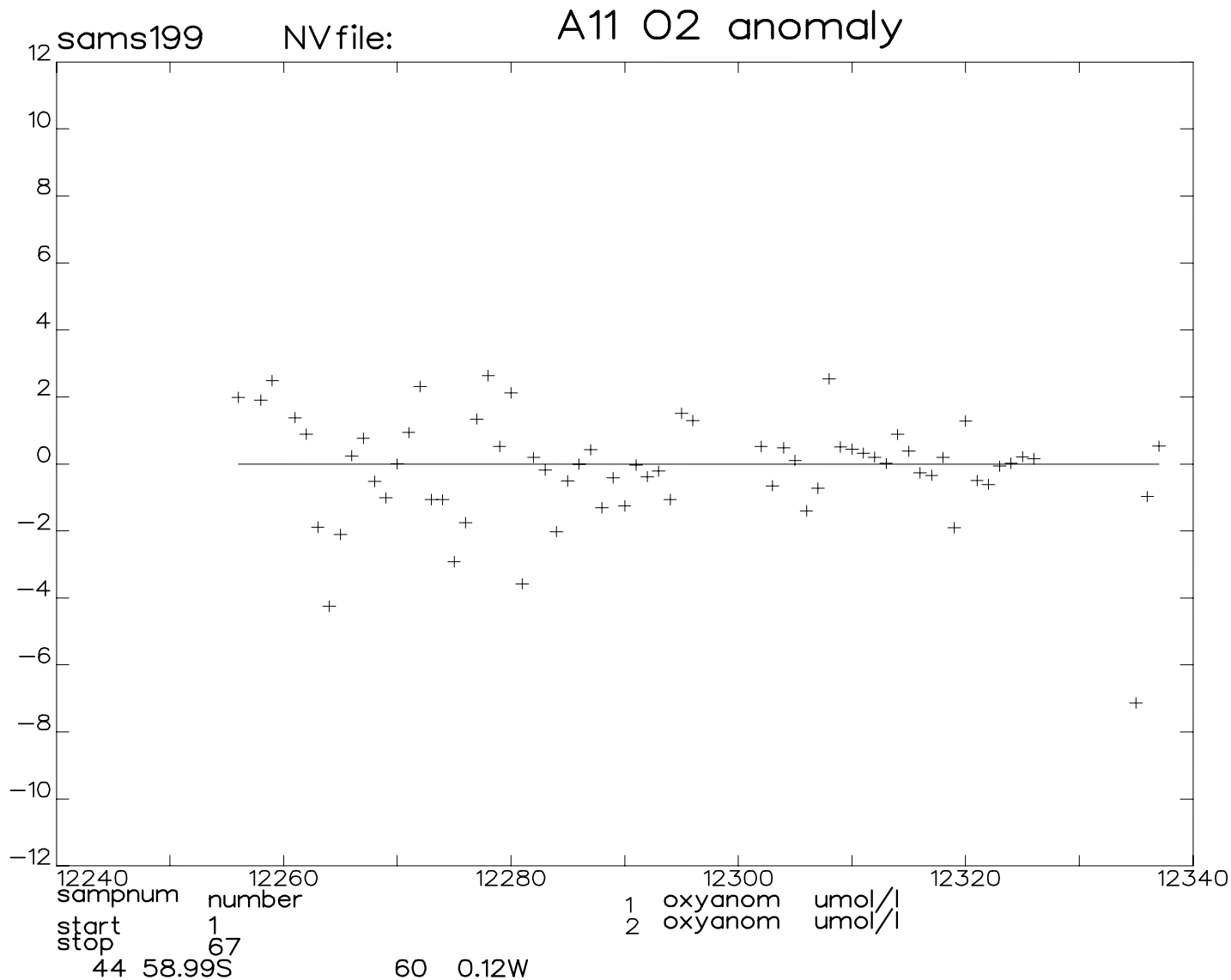
Figure 14: This cruise: station averages of anomaly of oxygen relative to standard fits. Horizontal axis: station number. Vertical axis: oxygen anomaly ( \mu\text{mol/l} ).
