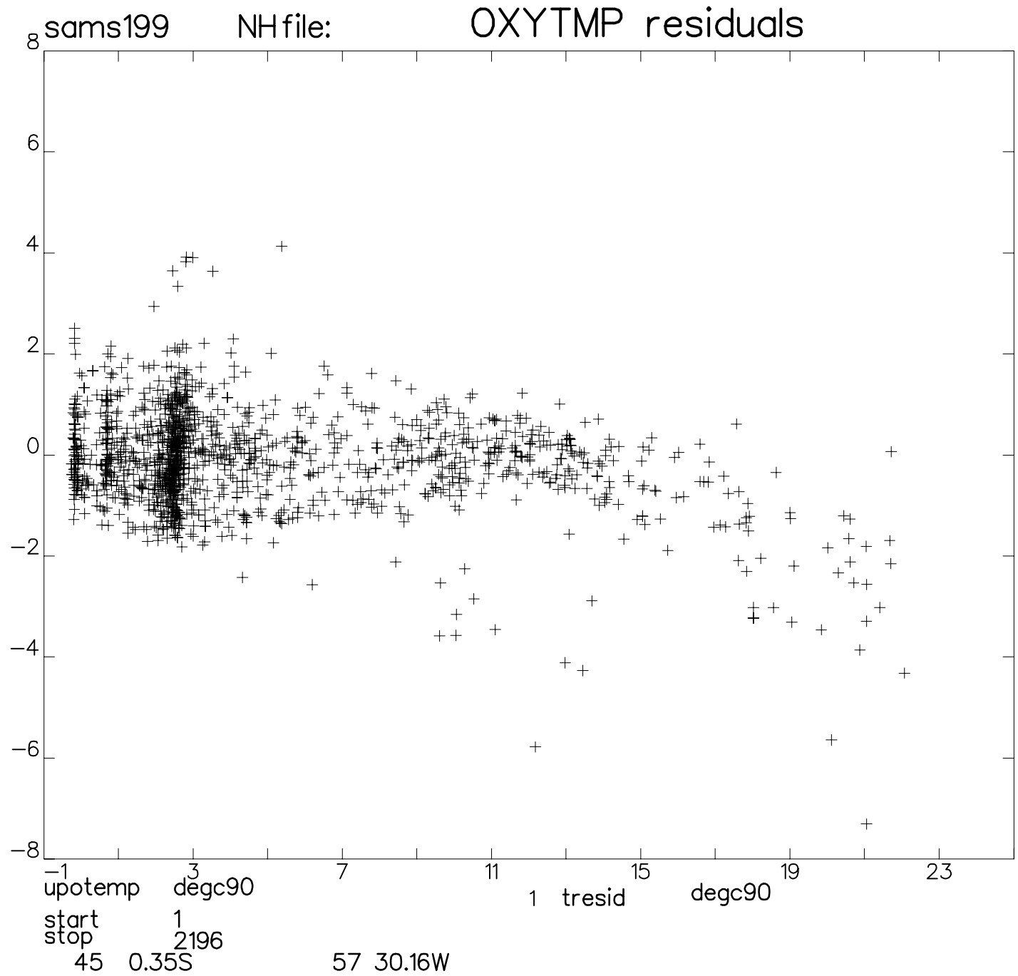
× Figure 13: This cruise: comparison of measured with predicted OXYTMP. Horizontal axis: THETA. Vertical axis: measured minus predicted OXYTMP.
