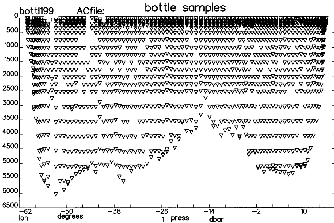
Figure 2: The location of 10 l water samples collected on cruise A11. Depth is in dbar.
