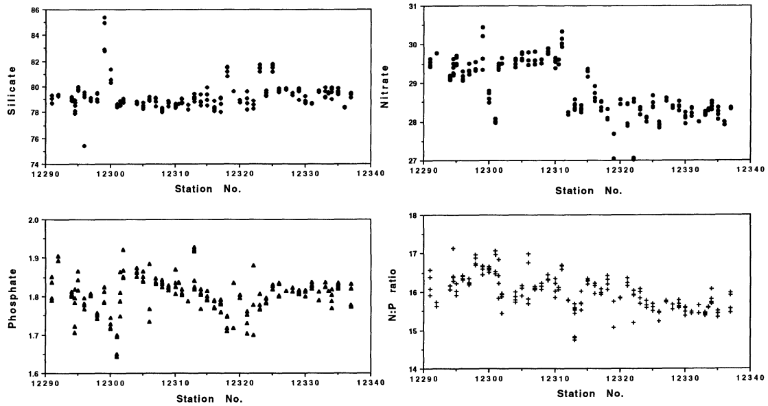
Figure 5: Deep water collected on station 12240 from 2500m was used as quality control for the nutrient measurements: results are shown for the last 50 stations of the cruise.
