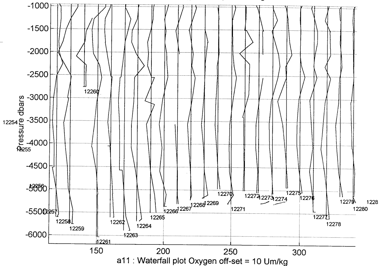
Figure 7a: CTD DQE
