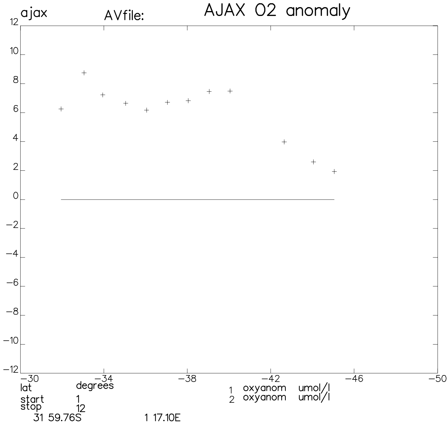
Figure 17: AJAX: station averages of anomaly of oxygen relative to standard fits. Horizontal axis: latitude. Vertical axis: oxygen anomaly ( \mu\text{mol/l} ). Intersects with A11 at 38 degrees south.
