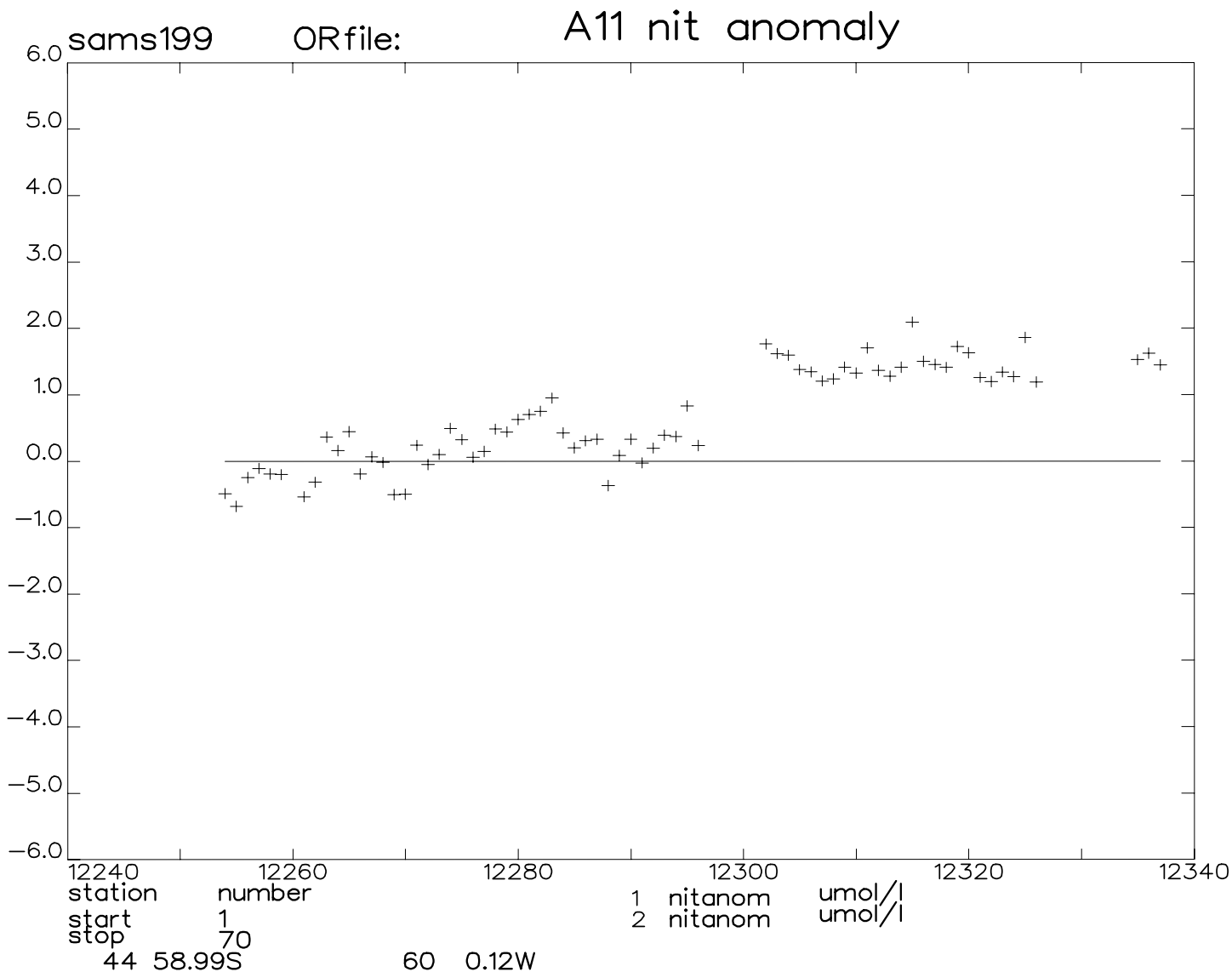
Figure 18a: Station averages of nitrate anomaly relative to standard fits. Horizontal axis: station number or latitude. Vertical axis: nitrate anomaly ( \mu\text{mol/l} ). 18a - This cruise. 18b - SAVE. 18c - AJAX.
