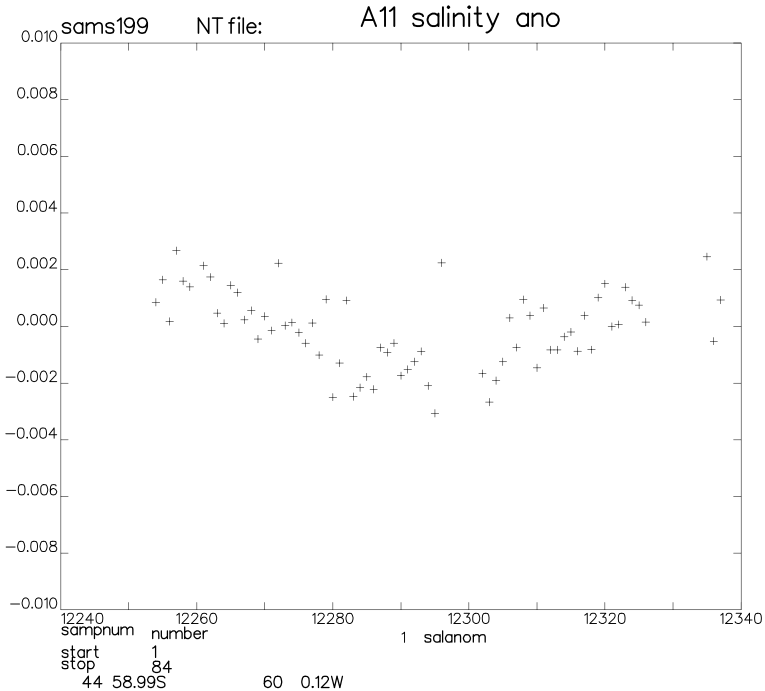
Figure 9: This cruise: station averages of anomaly of salinity relative to standard fits. Horizontal axis: station number. Vertical axis: salinity anomaly.
