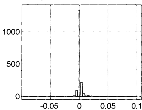
Figures 6a, 6b (top), 6c and 6d (bottom): CTD DQE
