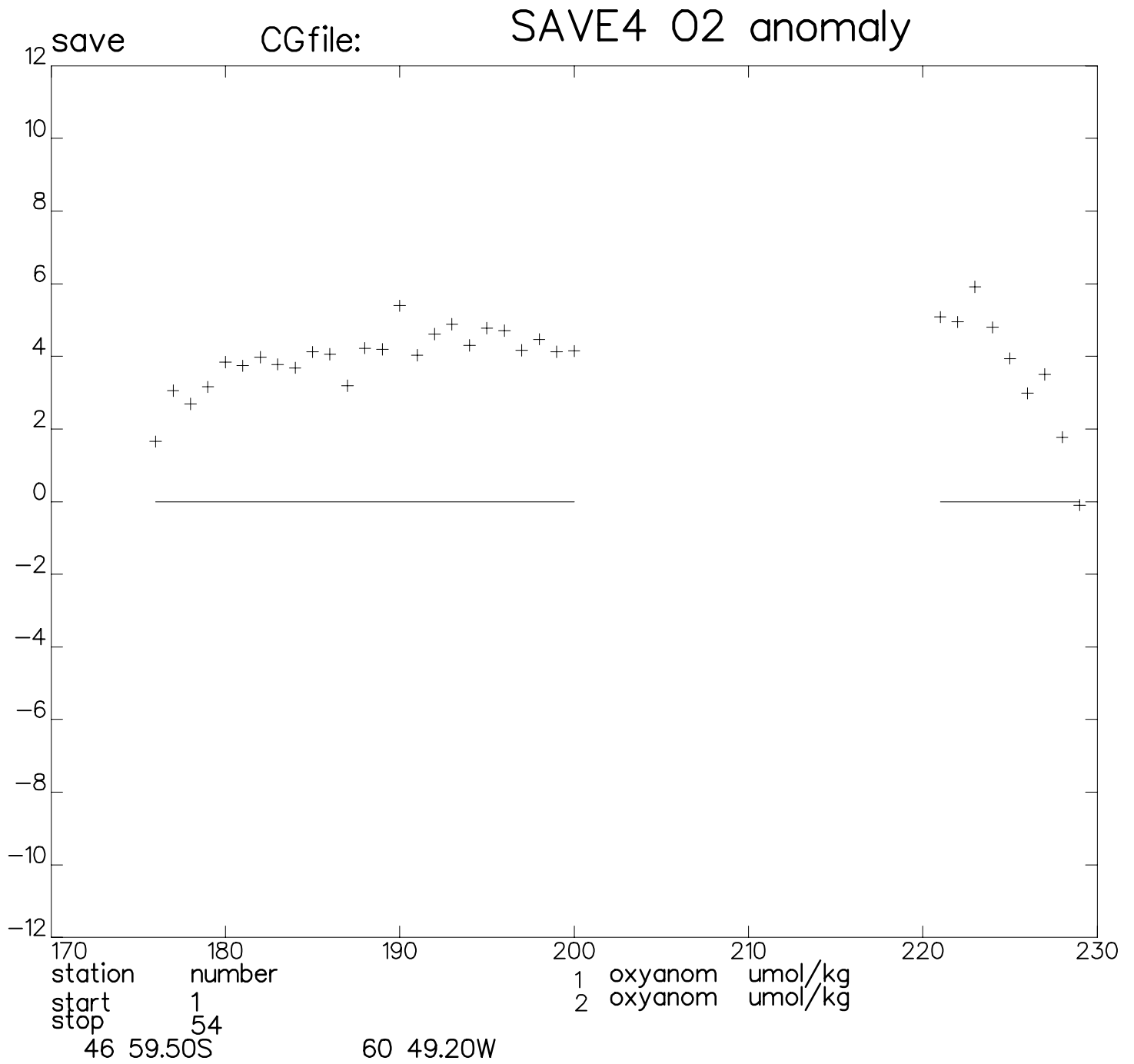
Figure 15: SAVE leg 4: station averages of anomaly of oxygen relative to standard fits. Horizontal axis: station number. Vertical axis: oxygen anomaly (μmol/kg).
