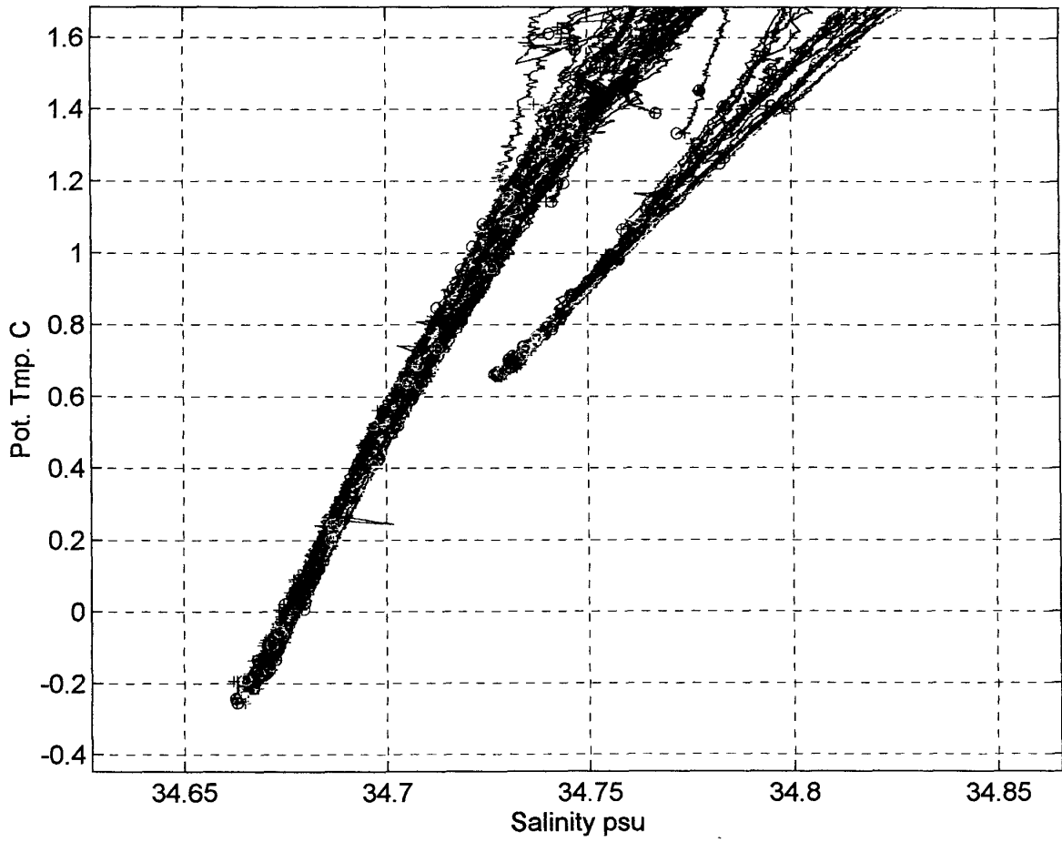
Figure 1b: CTD DQE
