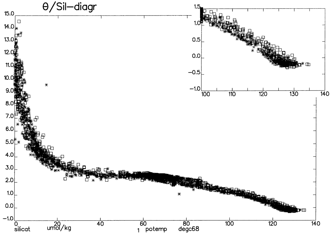
Figure 3: Silicate concentration versus potential temperature for A11 (*) and SAVE 4 data: both are in the Argentine basin and for the whole water column. The inset, for the deepest levels, shows the small discrepancy between the data sets.
