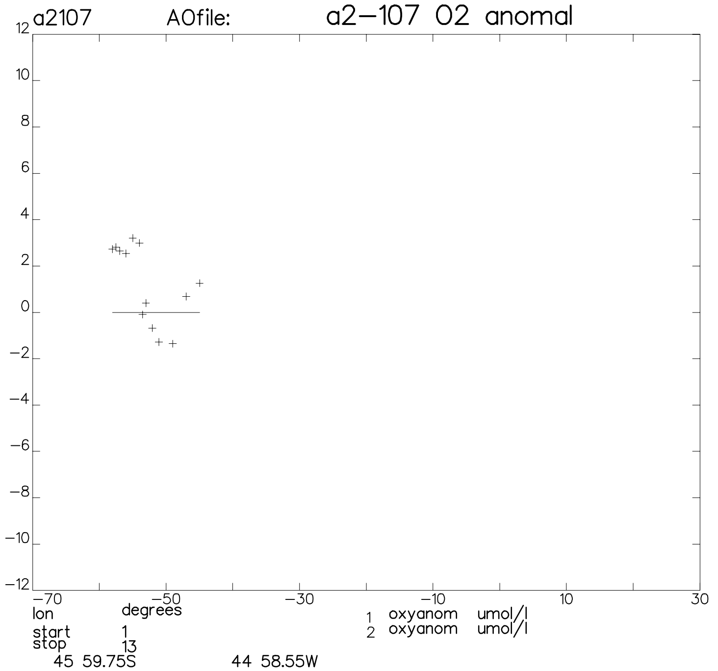
Figure 16: Atlantis II Cruise 107: station averages of anomaly of oxygen relative to standard fits. Horizontal axis: longitude. Vertical axis: oxygen anomaly ( \mu\text{mol/l} ).
