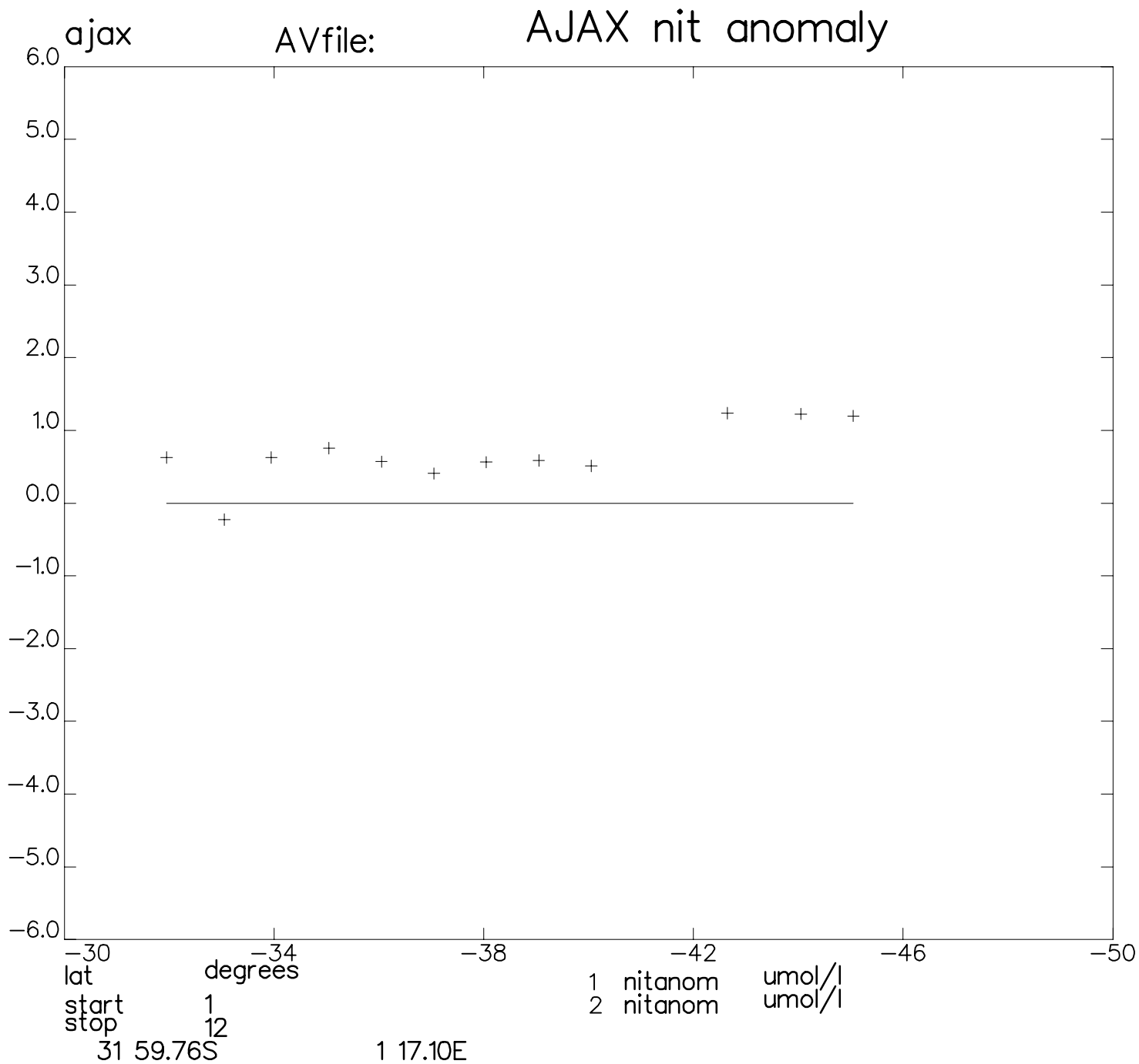
Figure 18c: Station averages of nitrate anomaly relative to standard fits. Horizontal axis: station number or latitude. Vertical axis: nitrate anomaly ( \mu\text{mol/l} ). 18a - This cruise. 18b - SAVE. 18c - AJAX.
