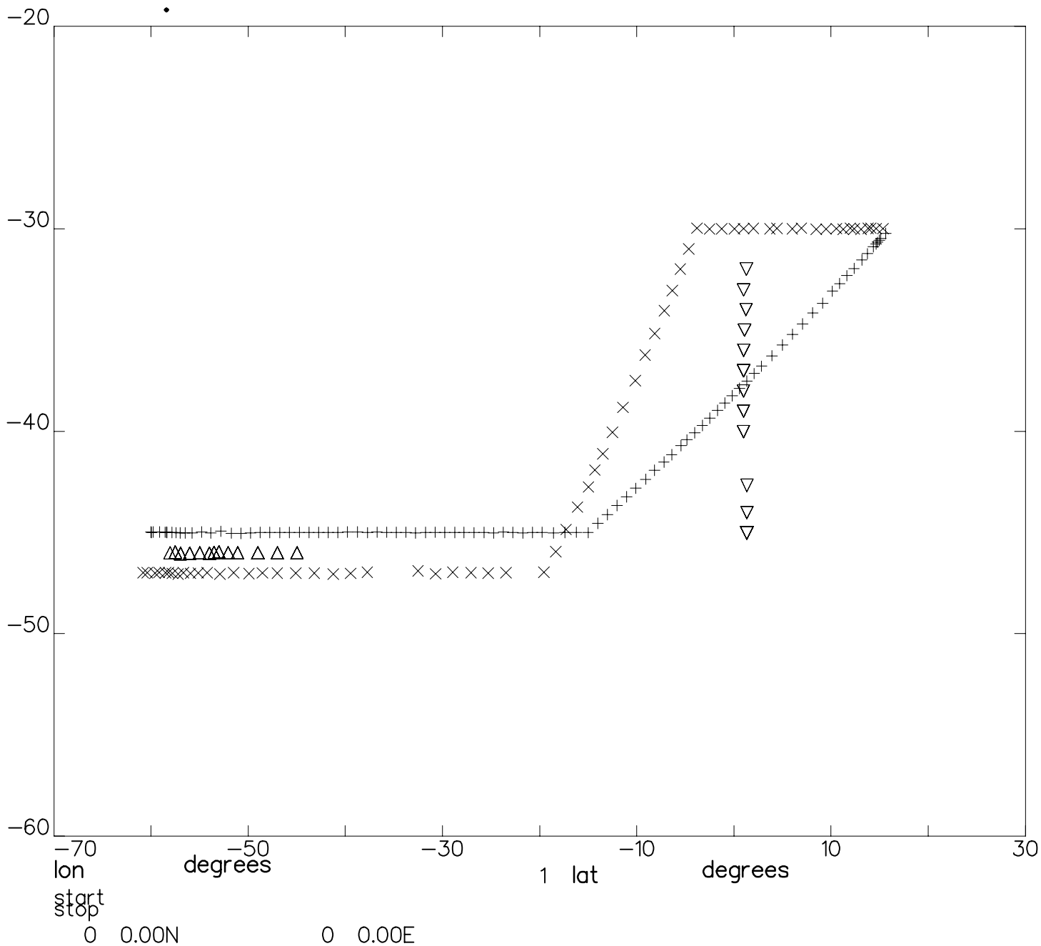
Figure 8: Location of A11 and historical data. Pluses, this cruise. Crosses, SAVE leg 4. Triangles, Atlantis II Cruise 107. Inverted triangles, AJAX.
