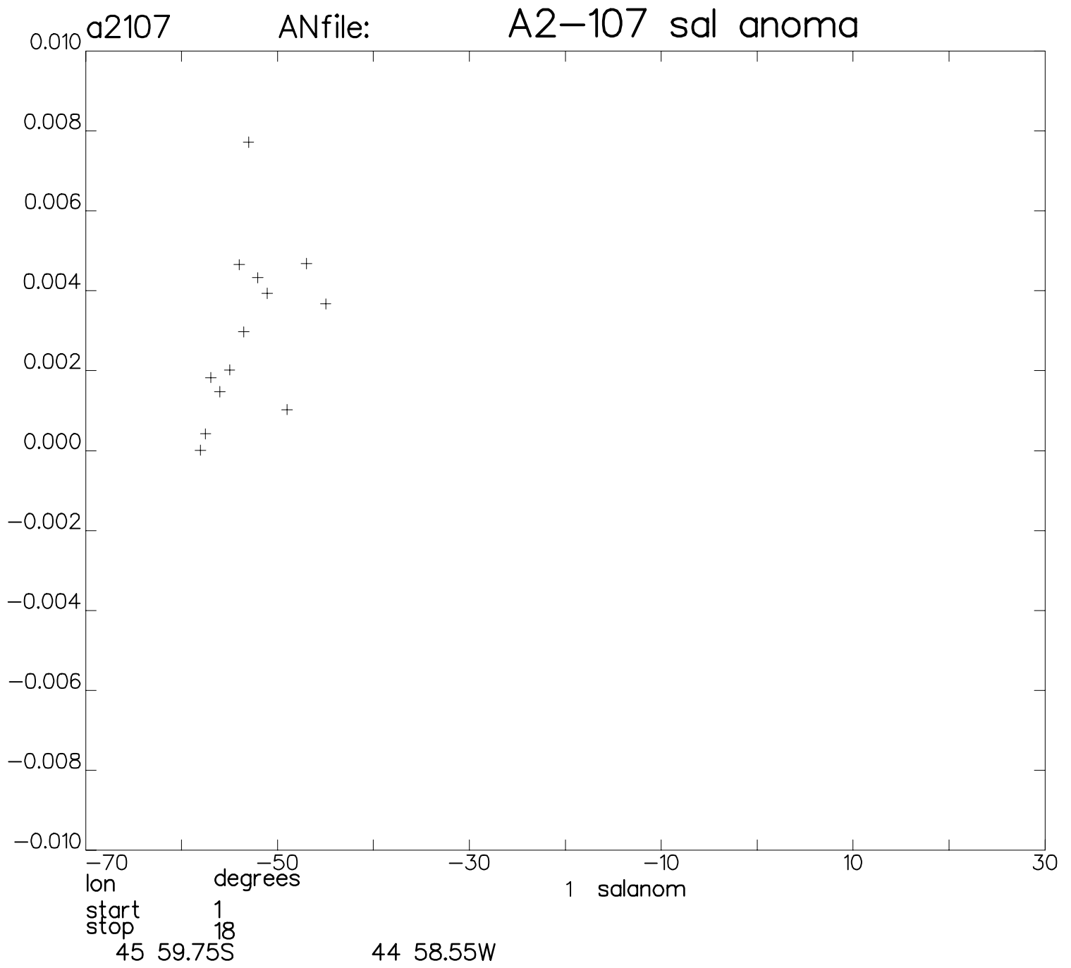
Figure 12: Atlantis II Cruise 107: station averages of anomaly of salinity relative to standard fits. Horizontal axis: longitude. Vertical axis: salinity anomaly.
