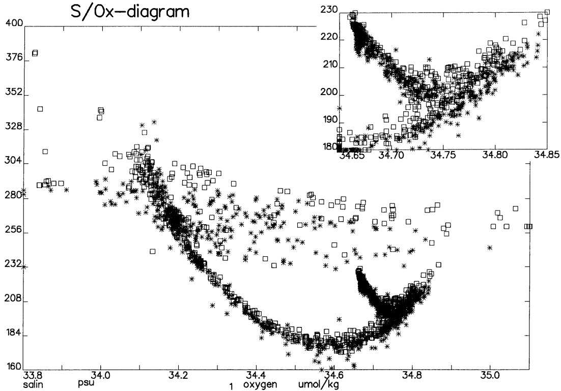
Figure 4: Dissolved oxygen concentration versus salinity for A11 (*) and SAVE 4 data: both are in the Argentine basin and for the whole water column. The inset, where the deepest levels form the left branch of the Y, shows the small discrepancy between the data sets.
