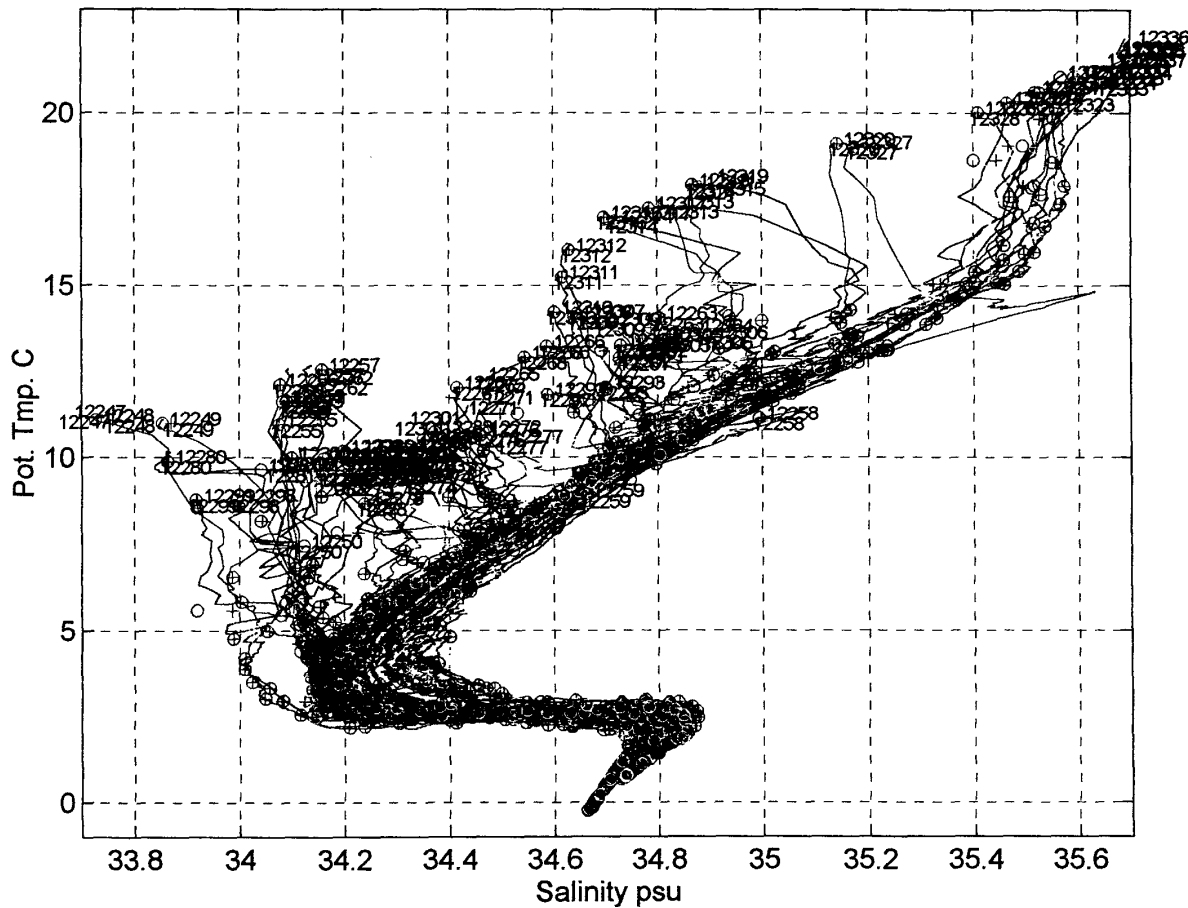
Figure 1a: CTD DQE
