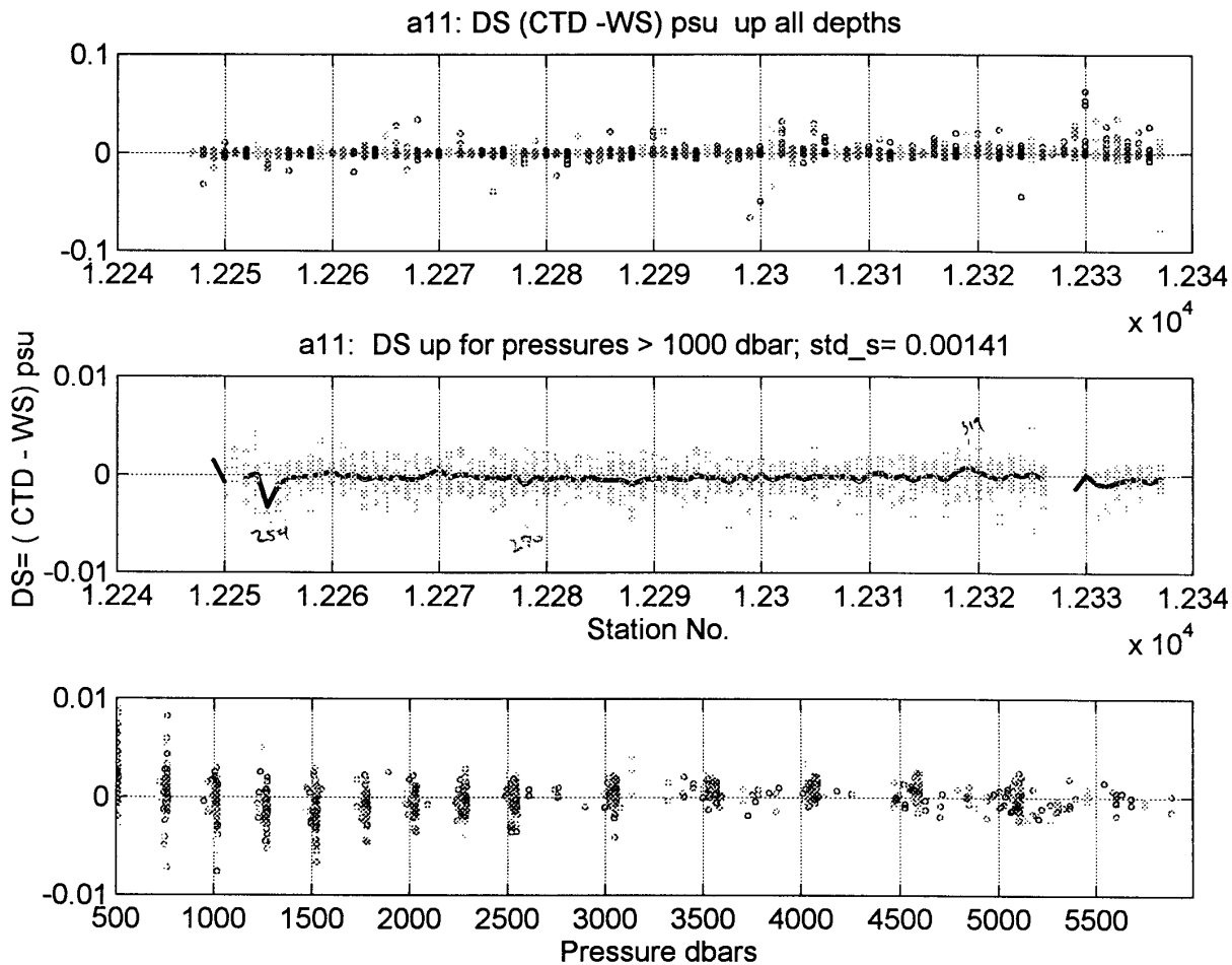
Figures 3a, 3b and 3c: CTD DQE
