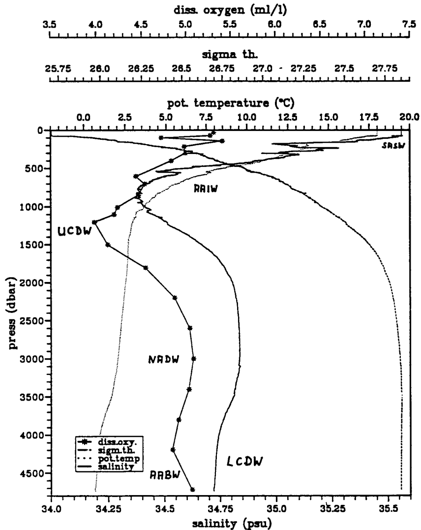
Fig. 2.1-5a: Profiles of potential temperature, salinity, dissolved oxygen, and density of station a) 542, and b) 601 which show some of the main water masses and their vertical extent in the Southern Ocean and the Weddell Gyre.
