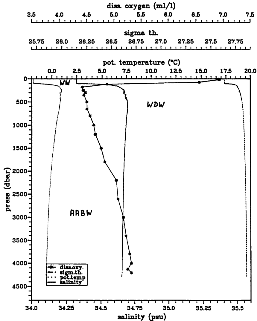
Fig. 2.1-5b: Profiles of potential temperature, salinity, dissolved oxygen, and density of station a) 542, and b) 601 which show some of the main water masses and their vertical extent in the Southern Ocean and the Weddell Gyre.
