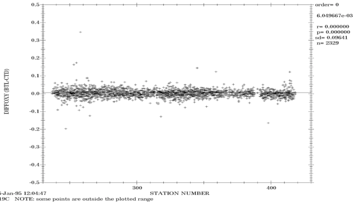
Figure 6b: P19C Residual Diss. Oxygen UpBottle-DownCTD Differences - Prs>1500dbar
