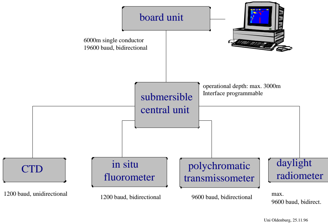
Fig. 7: Coupling of the optical sensors
