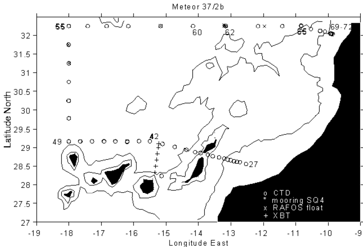
Fig 1: Station Map M37/2a (upper panel) and M37/2b (lower panel) with positions of CTD casts (o), moorings (*), and launched floats (x) and XBTs (+).
